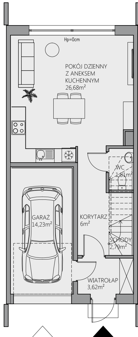
PLAN PARTERU
