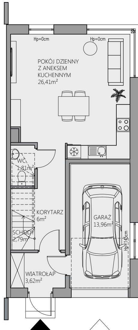
PLAN PARTERU
