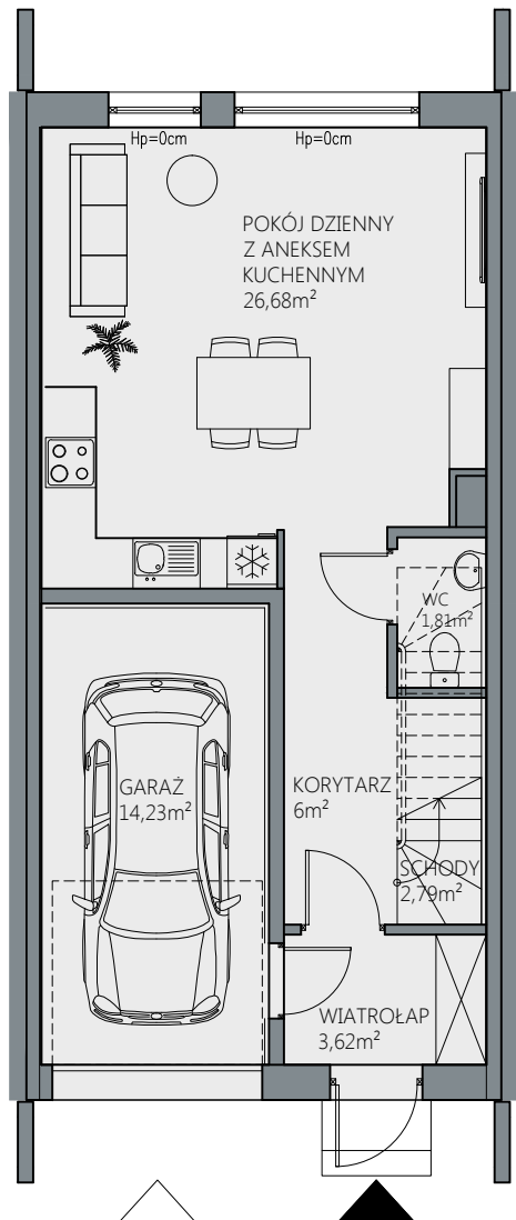
PLAN PARTERU
