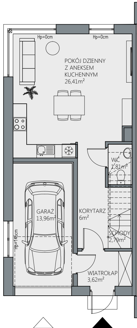
PLAN PARTERU
